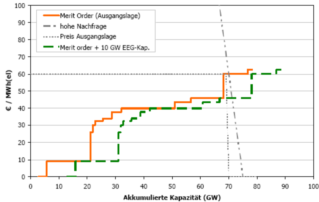
Figure 8: Impact of additional EEG capacity of 10 GW on the merit order
